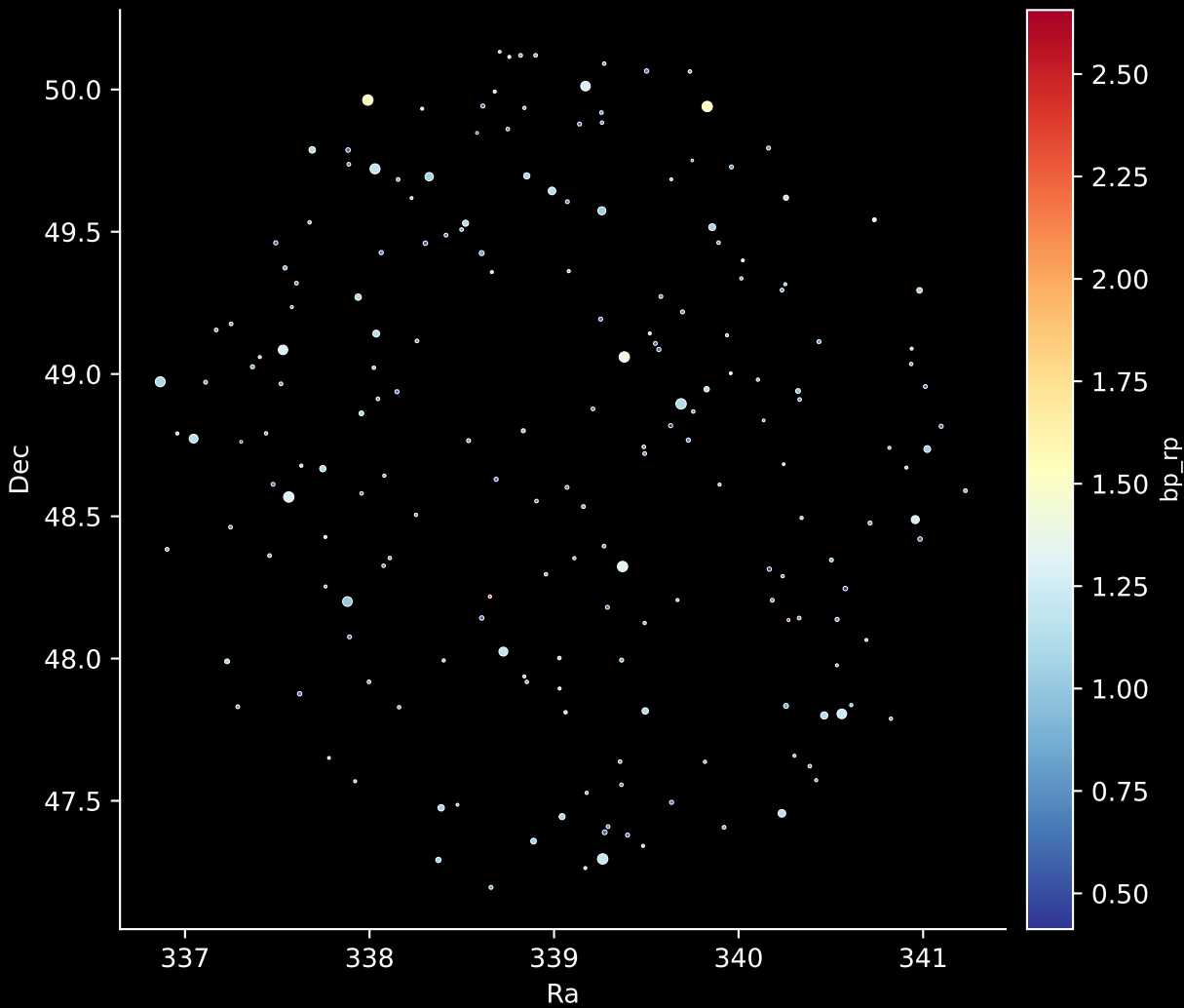
APOGEE DR17 Field: [077+49_MGA] Stars: 195
