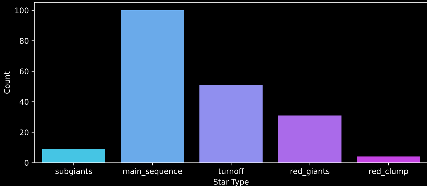
APOGEE DR17 Field: [077+49_MGA] Count plot of Star Type
