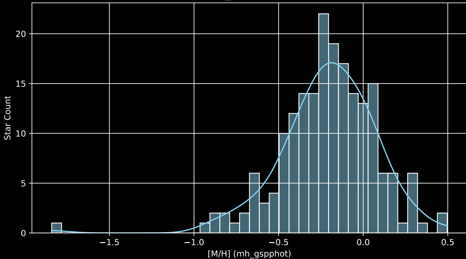
APOGEE DR17 Field: [077+49_MGA [M/H] (mh_gspphot) (n= 194)
