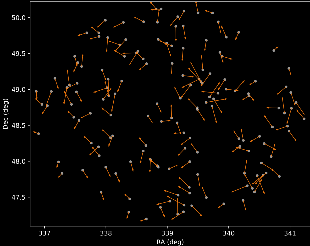
APOGEE DR17 Cluster 2 Proper Motion Vectors (n=152)
