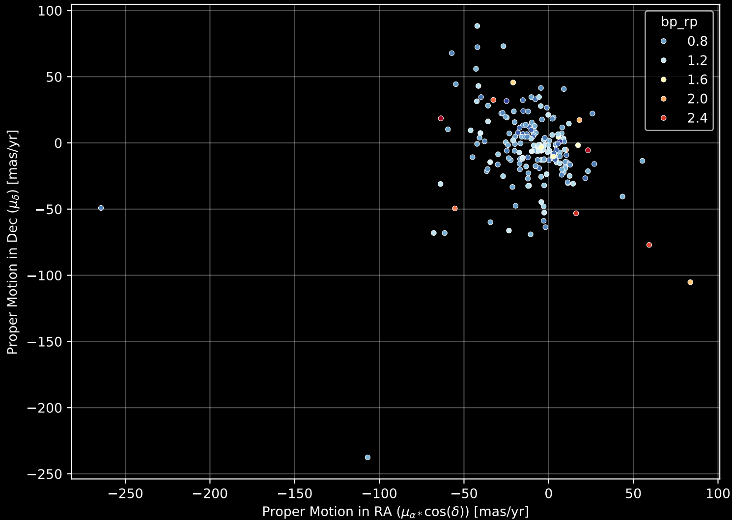
APOGEE DR17 Field: [077+49_MGA] Proper Motion Diagram (n= 195)
