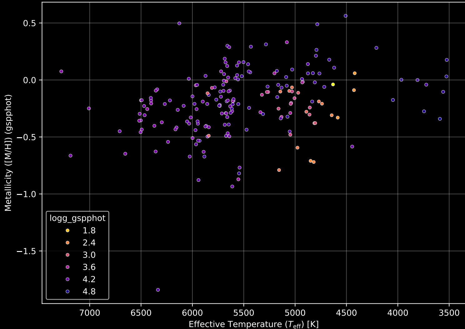
APOGEE DR17 Field: [077+49_MGA] Stellar Population Parameters (n= 195)
