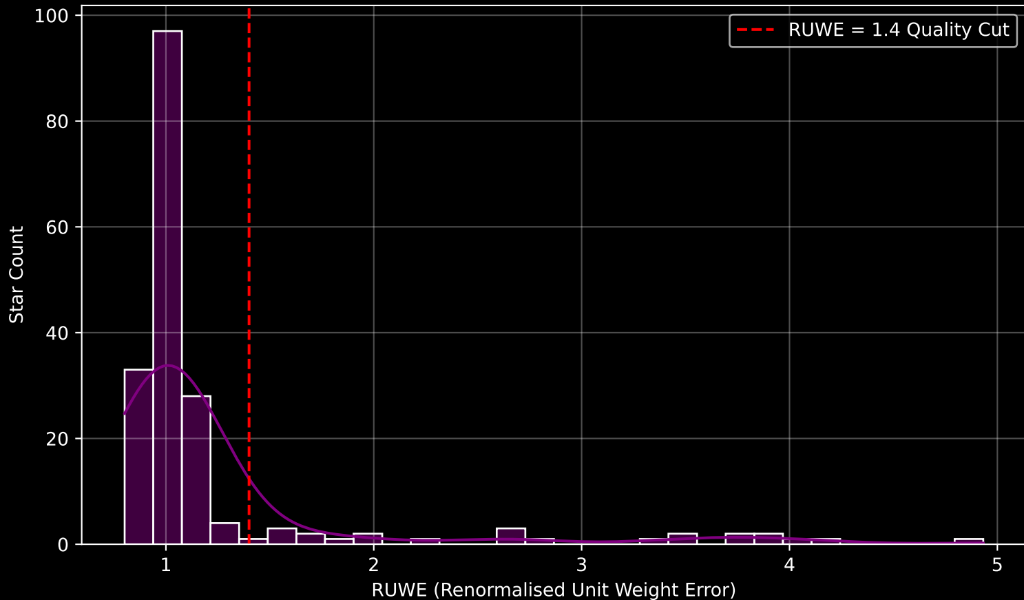
GAPOGEE DR17 Field [077+49_MGA] RUWE Distribution (n= 186)
