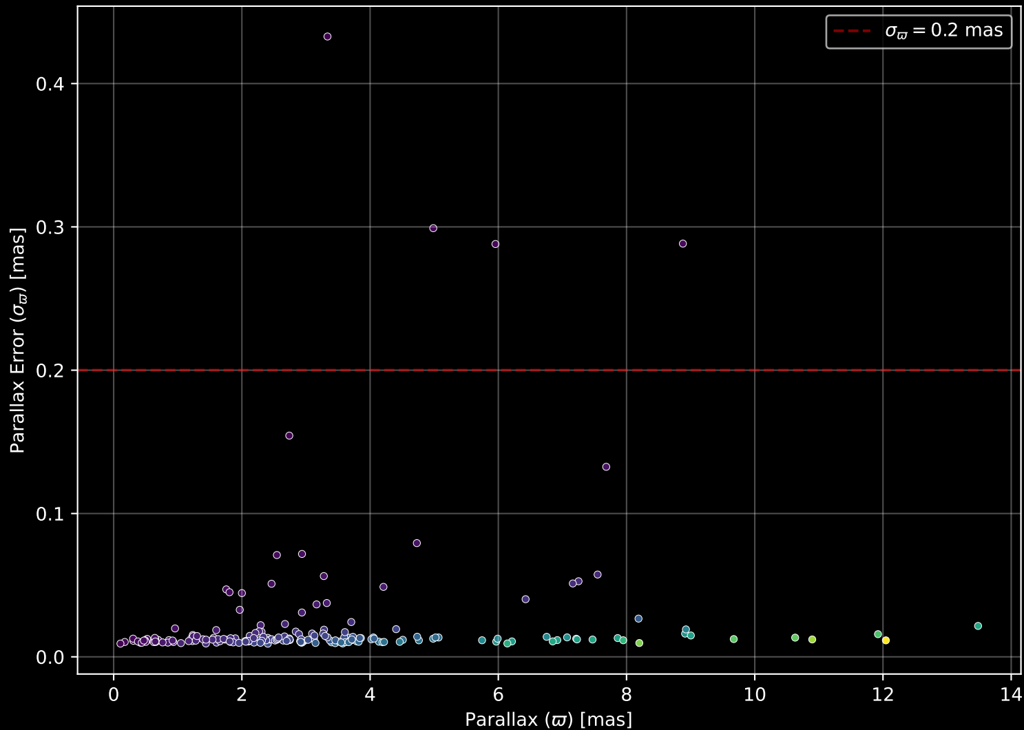
APOGEE DR17 Field: [077+49_MGA] Parallax Quality (n= 195)
